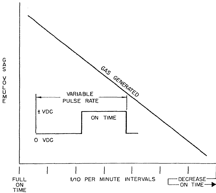
GAS GENERATED VS. PULSE VOLTAGE RATE
